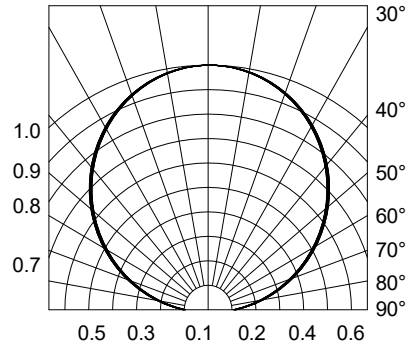
Fig.6-Radiation Diagram Ta=25°C
