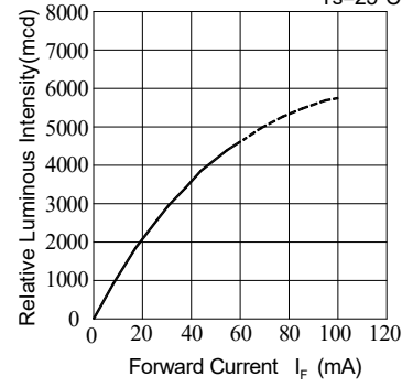
Fig.2-Relative Luminous Intensity vs. Forward Current Ts=25°C
