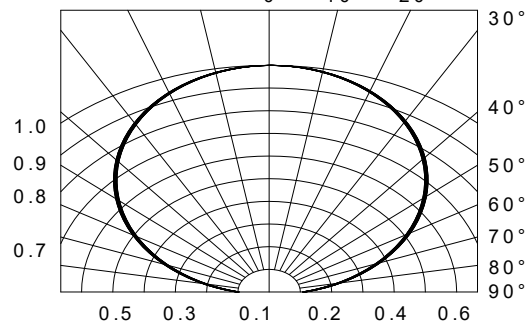
Fig.6-Radiation Diagram Ta=25°C
