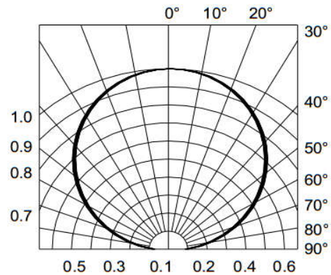
Fig.6-Radiation Diagram Ta=25°C
