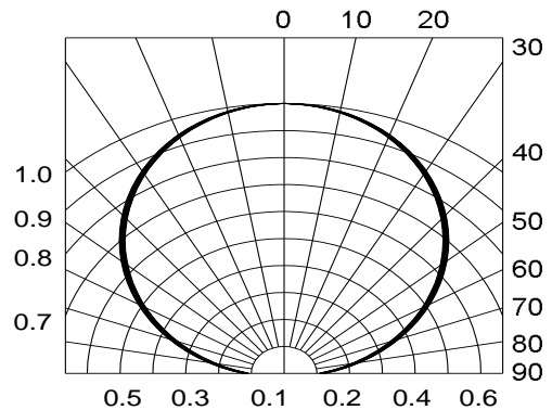
Fig.6-Radiation Diagram Ta=25 C
