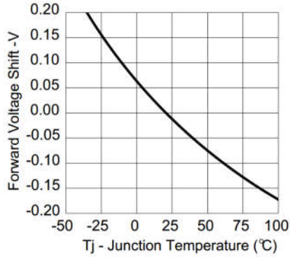
Fig.1 - Forward Voltage Shift vs. Junction Temperature
