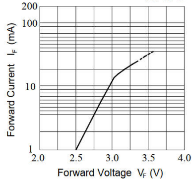
Fig.4-Forward Current vs. Forward Voltage Ta=25°C
