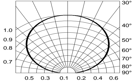
Fig.6-Radiation Diagram Ta=25°C
