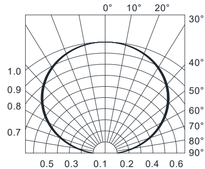
Fig.6-Radiation Diagram Ta=25°C
