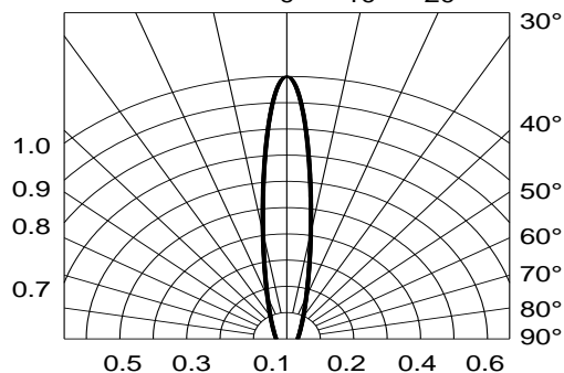
Fig.6-Radiation Diagram Ta=25°C
