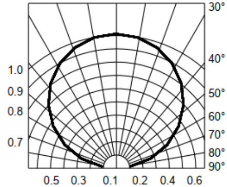
Fig.6-Radiation Diagram Ta=25°C
