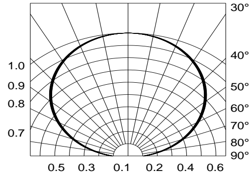
Fig.6-Radiation Diagram Ta=25°C
