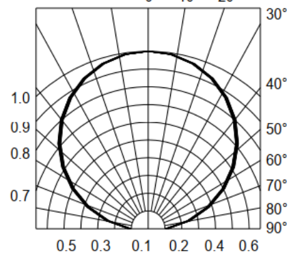
Fig.6-Radiation Diagram Ta=25°C
