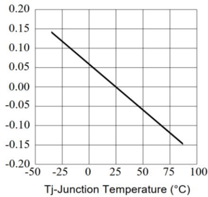
Fig.1-Forward Voltage Shift vs. Junction Temperature
