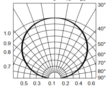
Fig.6-Radiation Diagram Ta=25°C
