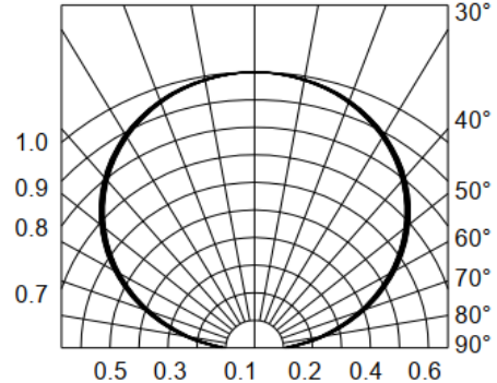
Fig.6-Radiation Diagram Ta=25°C
