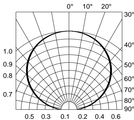
Fig.6-Radiation Diagram Ta=25°C
