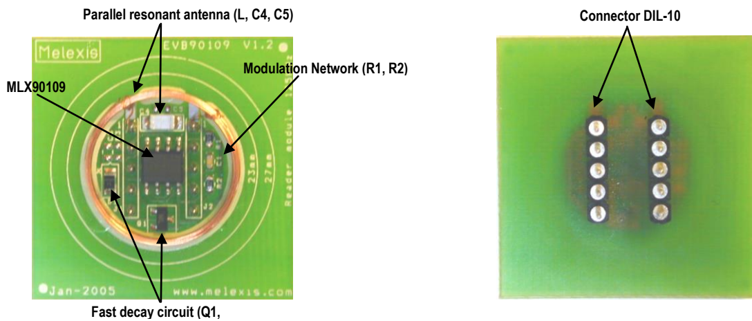
Figure 1: EVB90109
