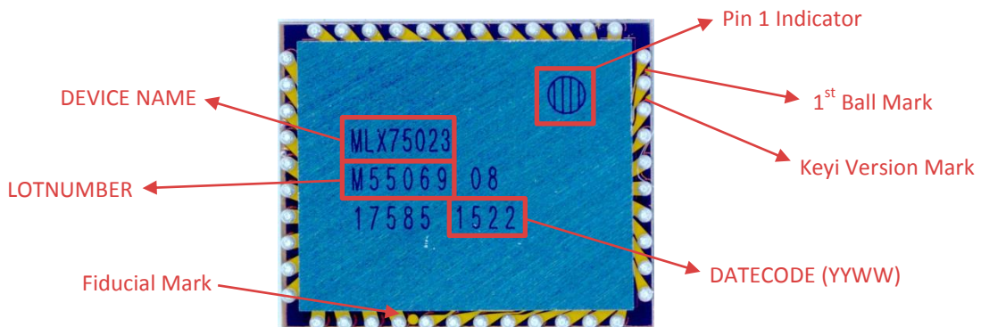
Figure 11: Contrast Enhanced Picture of Sensor Backside
