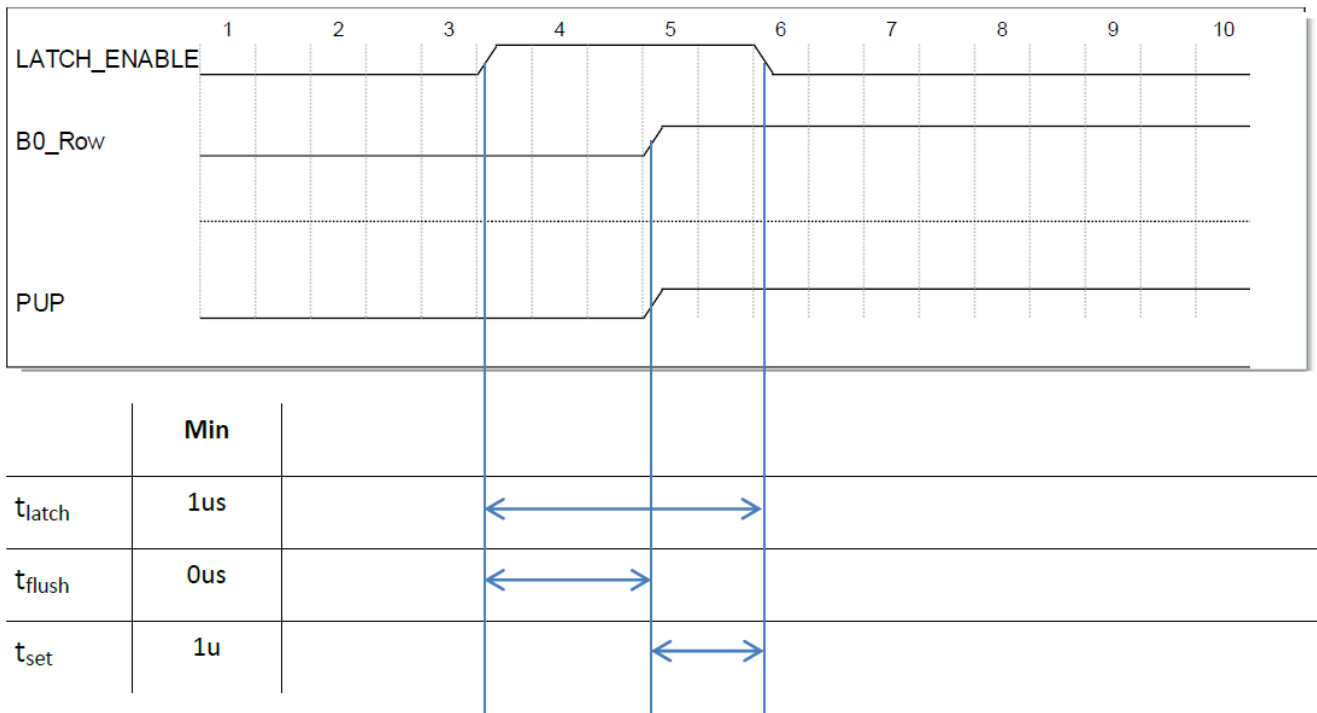
Figure 6: Device control
