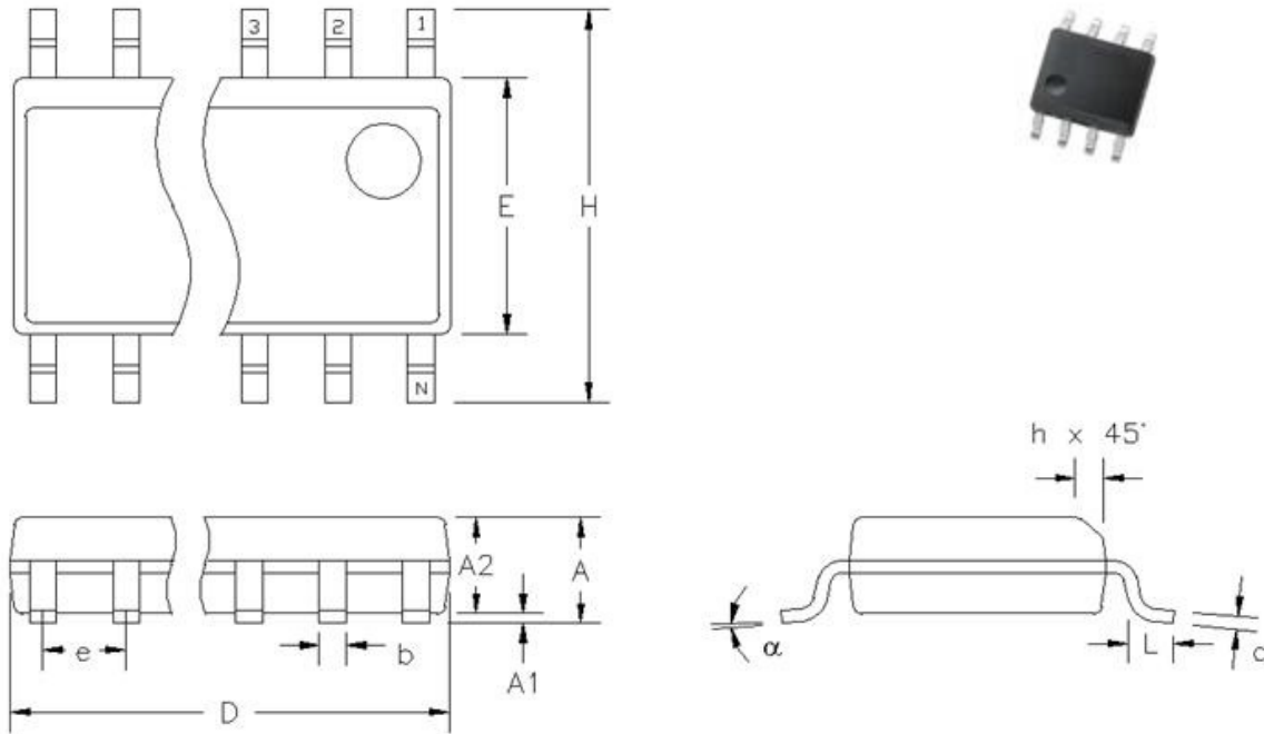
Figure 6: Package drawing
