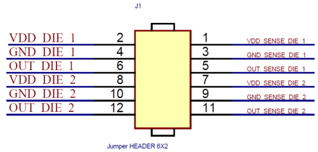
Figure 6: Jumper between force and sense line.
