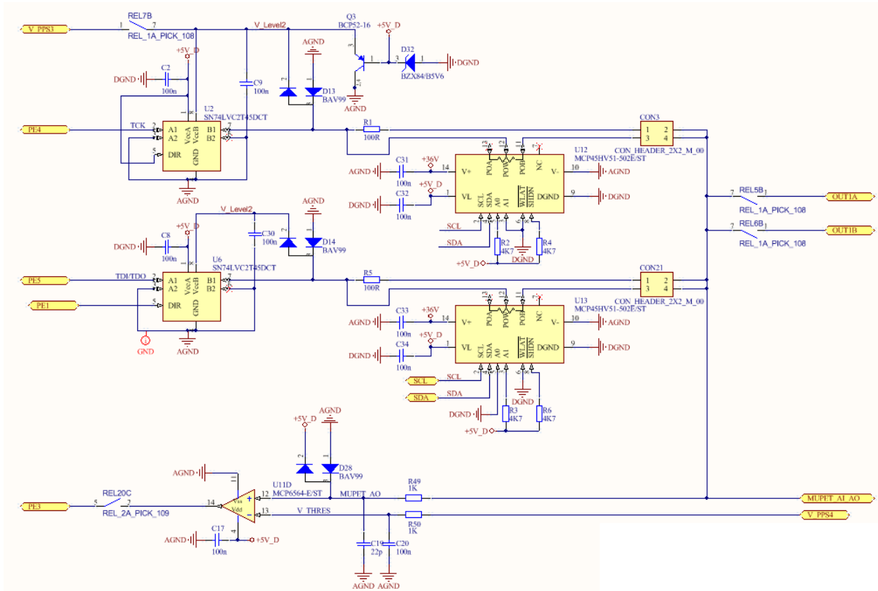
Figure 8: MUPET Block
