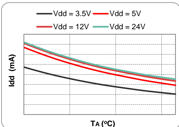
11.5. I_{DD} vs. T_A
