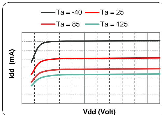
11.6. I_{DD} vs. V_{DD}
