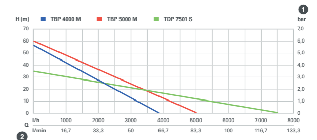
Deep Well Pumps / Submersible Pressure Pumps
