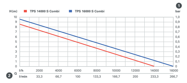
Dirty Water Submersible Pumps
