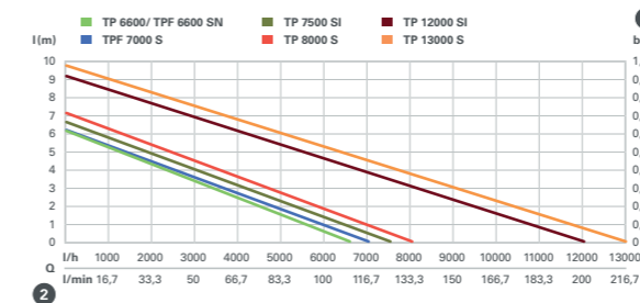
Construction and Dirty Water Pumps
