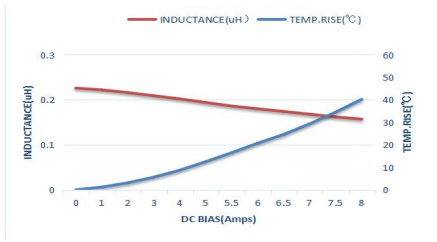
MTQH201210SR33MBT
