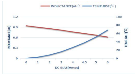
MTQH201610S1R0MBT
