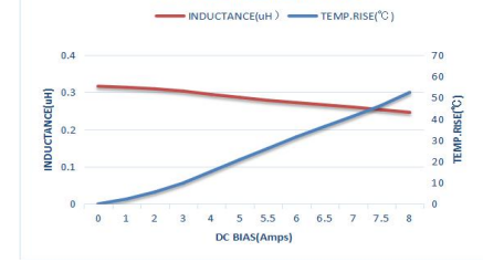
MTQH252012SR33MBT
