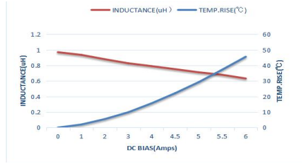
MTQH252010S1R0MBT
