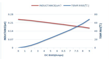
MTQH252010SR24MBT
