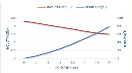
MTQH252012S2R2MBT
