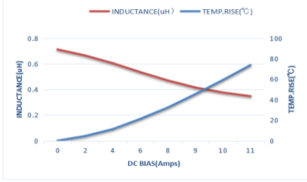
MTQH252012SR68MBTA
