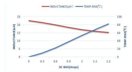
MTQH252010S220MBT
