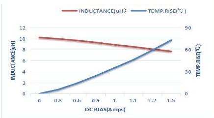
MTQH252010S100MBT
