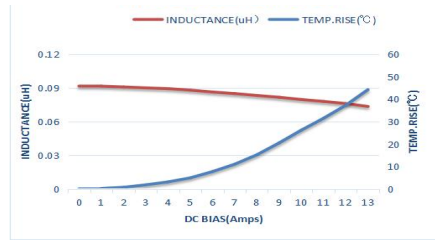
MTQH252012SR10MBT
