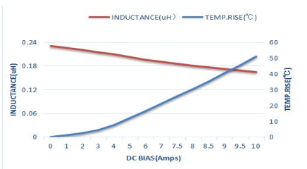
MTQH252012SR22MBT
