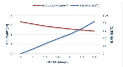
MTQH252012SR10MBT
