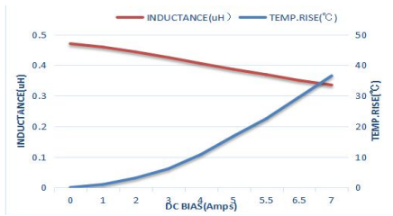
MTQH252010SR47MBTA
