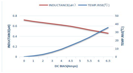
MTQH252010SR68MBT
