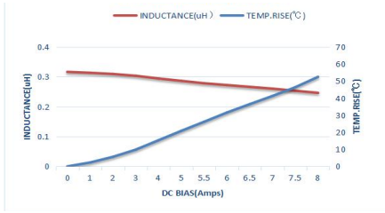
MTQH252012SR33MBT
