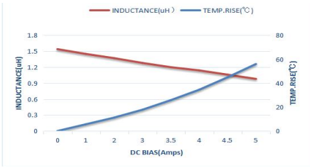
MTQH252010S4R7MBT
