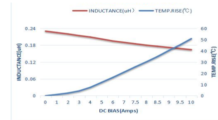
MTQH252012SR24MBT
