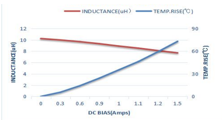
MTQH252010S100MBT
