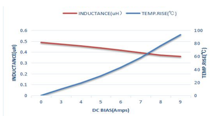
MTQH322510SR47MBT
