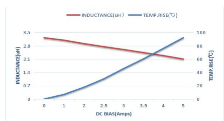
MTQH322512S100MBT
