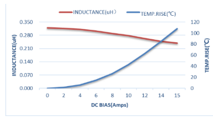
MTQH322520S1R0MBT
