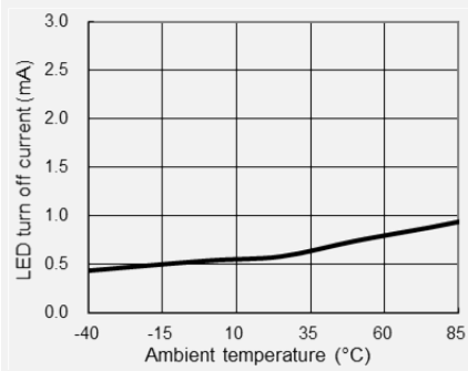
LED turn off current vs. ambient temp.
