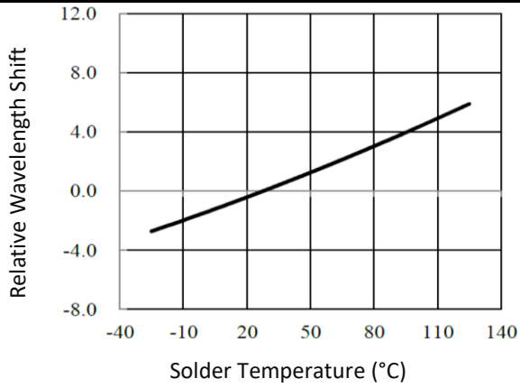
Wavelength Shift v.s. Solder Temperature
