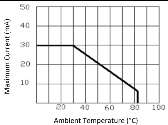
Max. Forward Current v.s. Ambient Temp.
