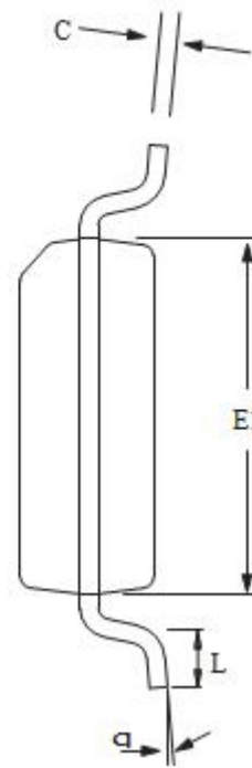
End View
