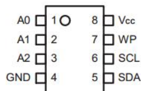
8 - lead SOP
