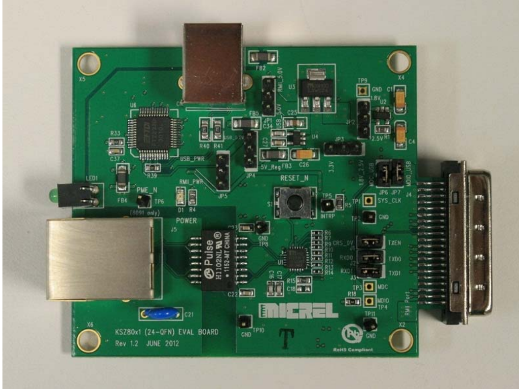
Figure 1. KSZ8081RNA / KSZ8081RND Evaluation Board
