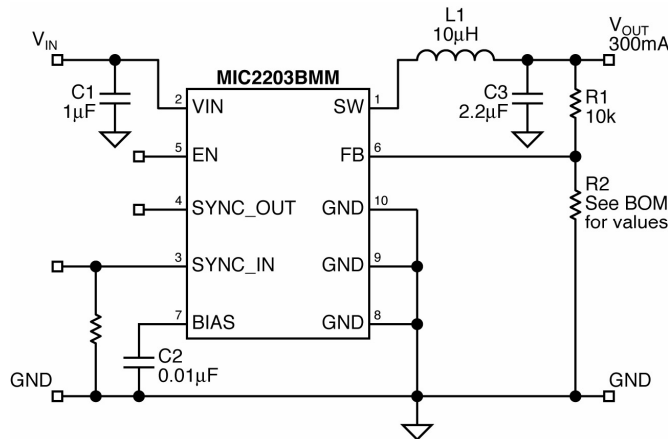
Figure 2. MIC2203BMM Evaluation Board Schematic
