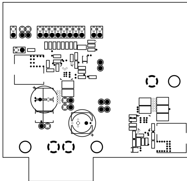
Mid-Layer 1 (Power Ground Plane)
