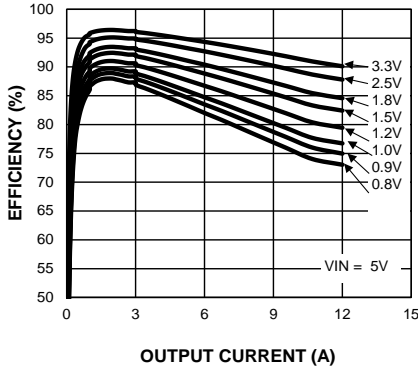
Efficiency (VIN = 5V) vs. Output Current
