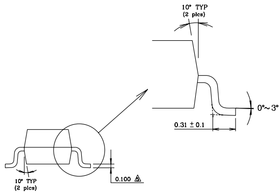
END VIEW
