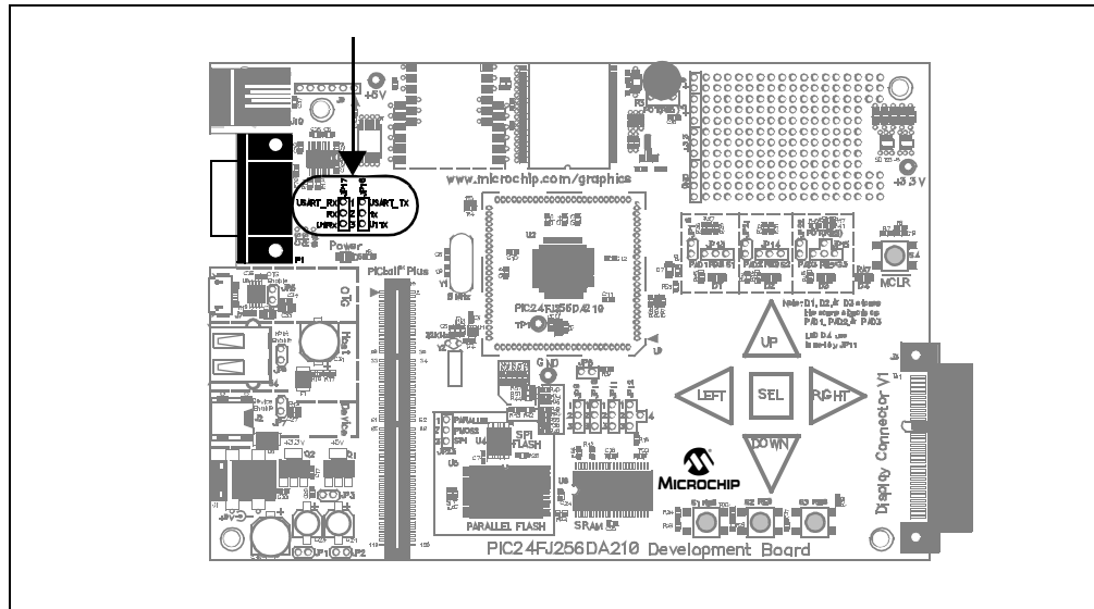
FIGURE 4-5: UART CONFIGURATION
