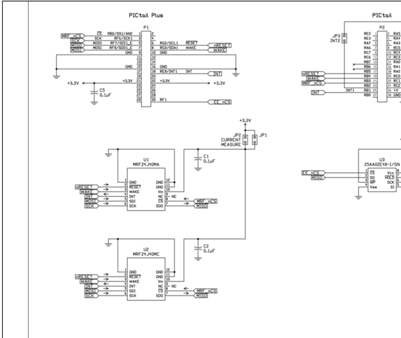
FIGURE A-1: MRF24J40MC PICtail™/PICtail PLUS DAUGHTER BOARD SCHEMATIC
