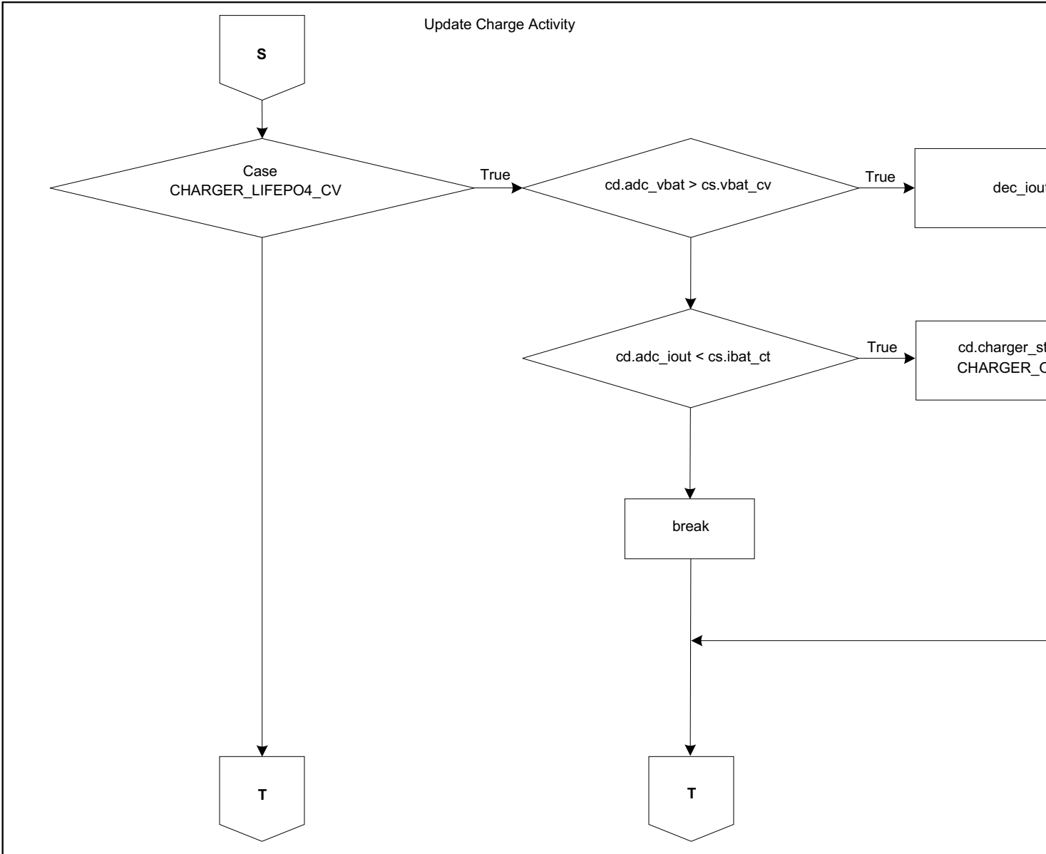
FIGURE C-16: Block Diagram of LiFEPO4 Profile Termination.
