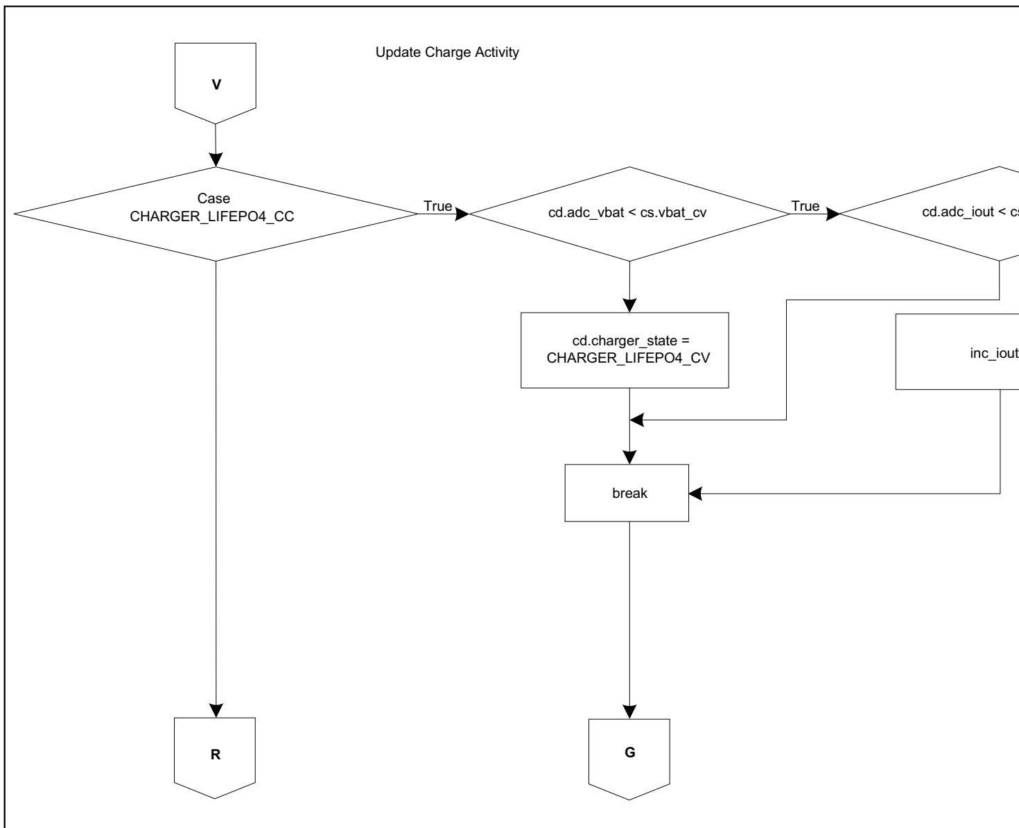
FIGURE C-15: Block Diagram of Transition to LiFEPO4 Constant-Current Charging Mode.
