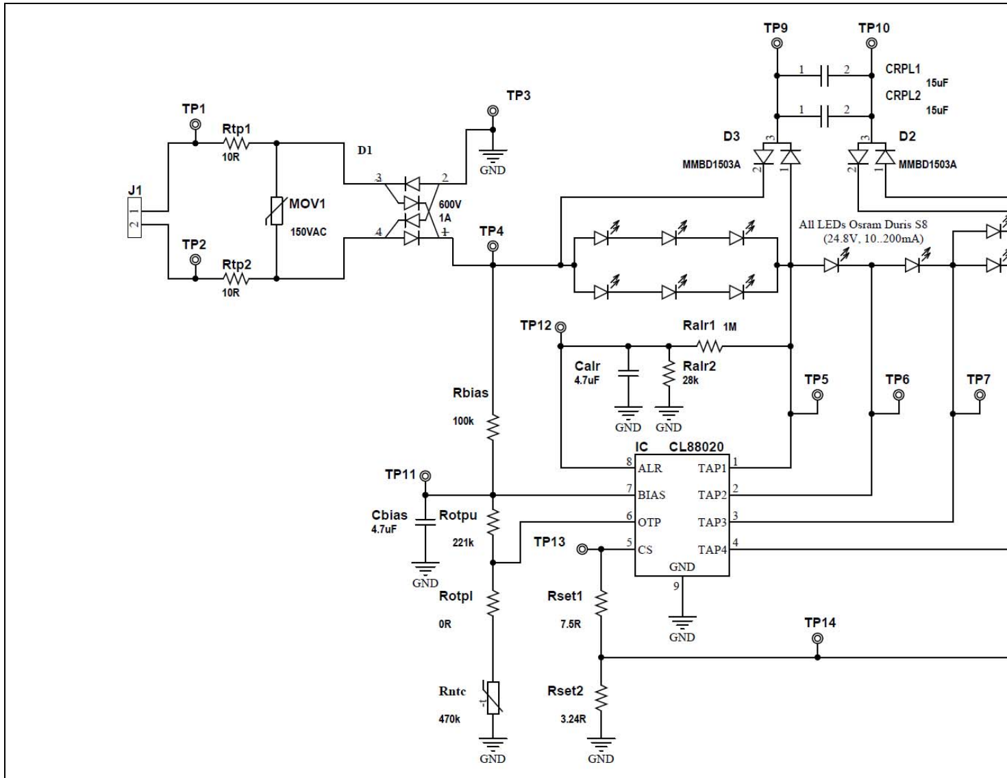
FIGURE 1-1: Typical CL88020 120 V AC Offline LED Driver Evaluation Board Circuit.
