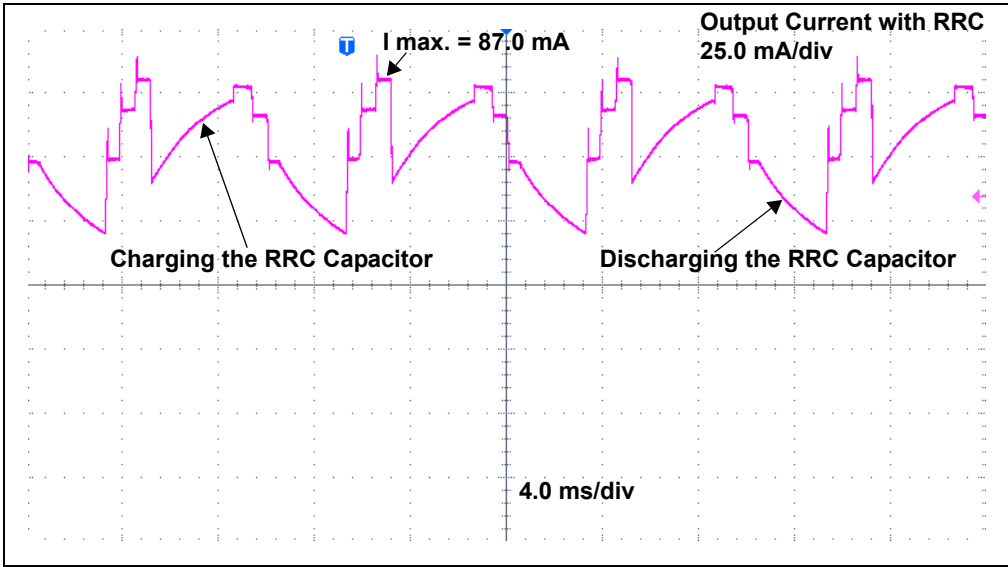
FIGURE C-11: Output Current with RRC at 230 V AC Line Input Voltage.
