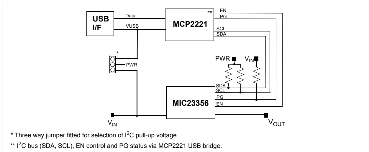
FIGURE 2-1: MIC23356 Step-Down Regulator with MCP2221 I 2 C Bridge.
