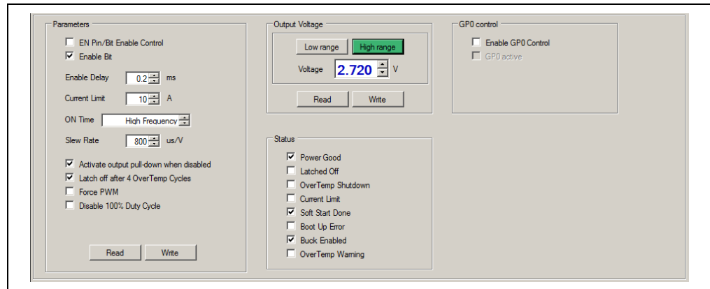
FIGURE 4-7: MIC23356 I 2 C Programmable Features Area – High Range.
