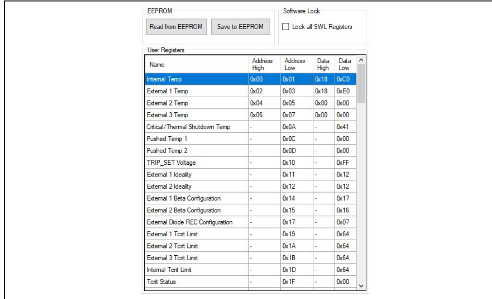
FIGURE 3-17: Registers List Tab.
