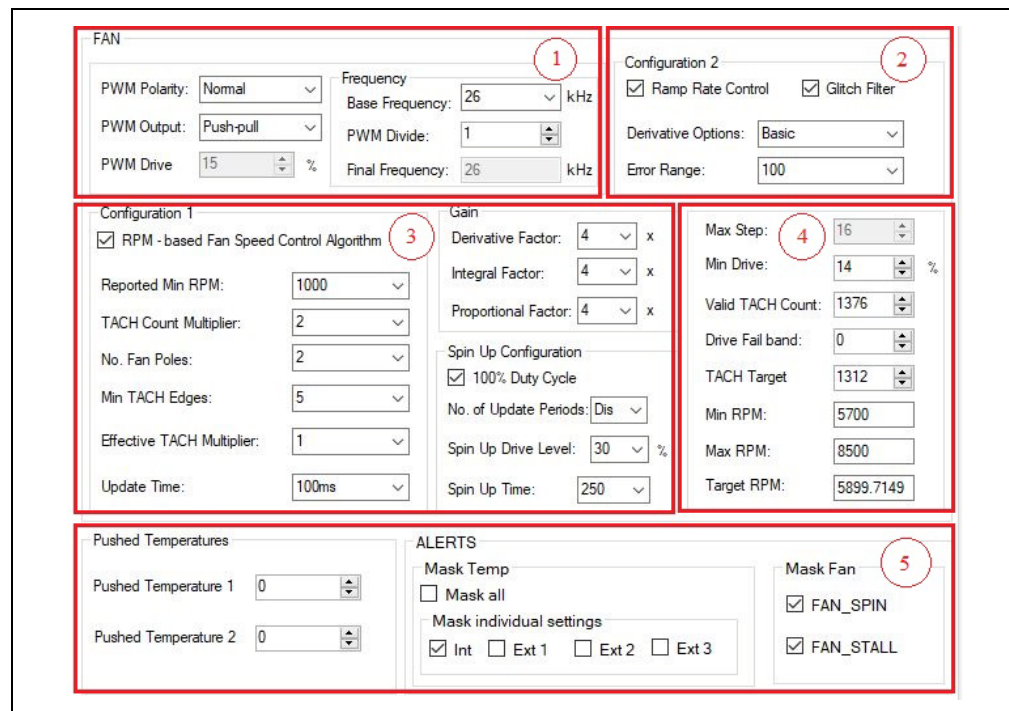
FIGURE 3-19: Fan Driver Tab.
