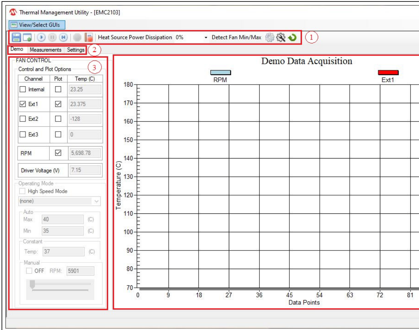
FIGURE 3-2: Thermal Management Utility Main Window.
