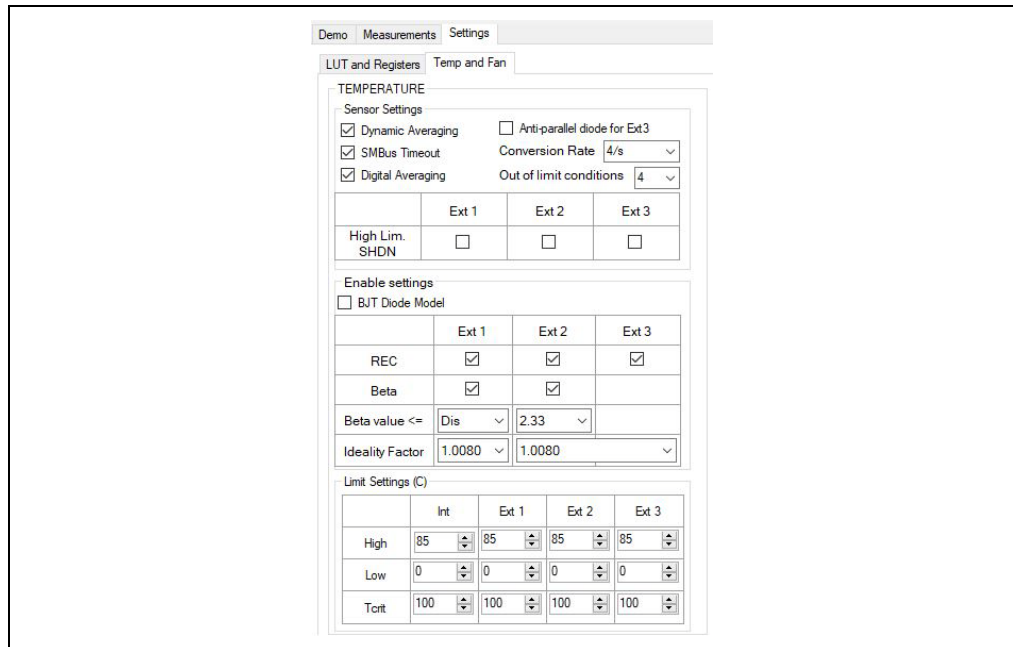
FIGURE 3-18: Temperature Sensor.
