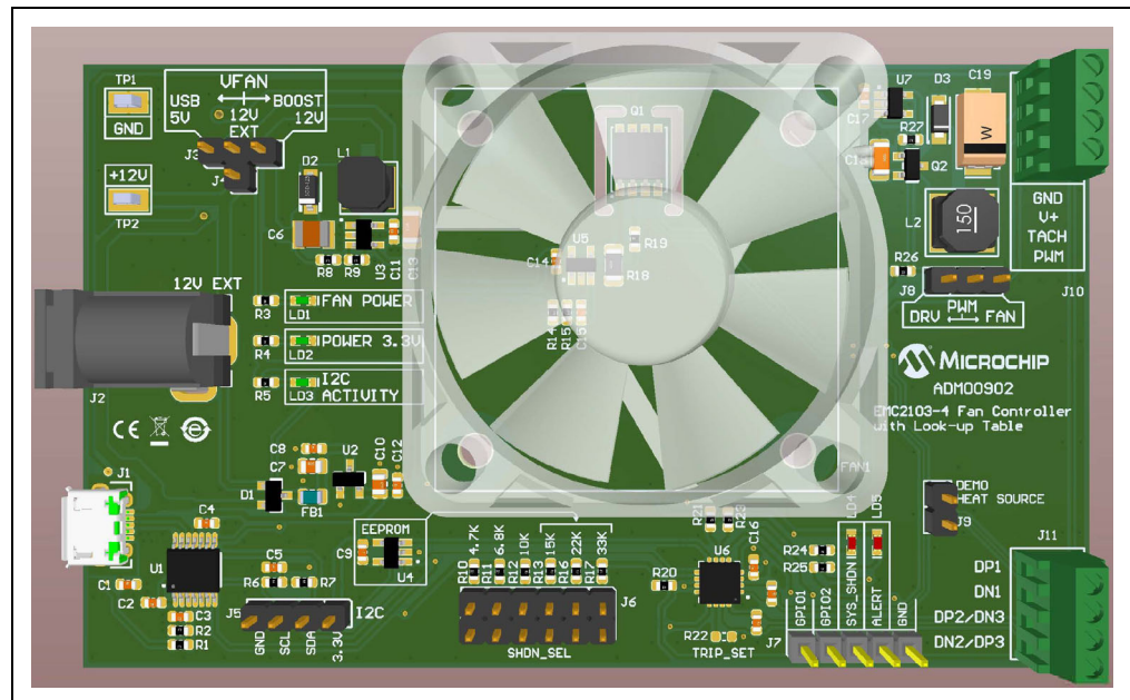
FIGURE 4-1: ADM00902 Demonstration Board for EMC2103 Top View.
