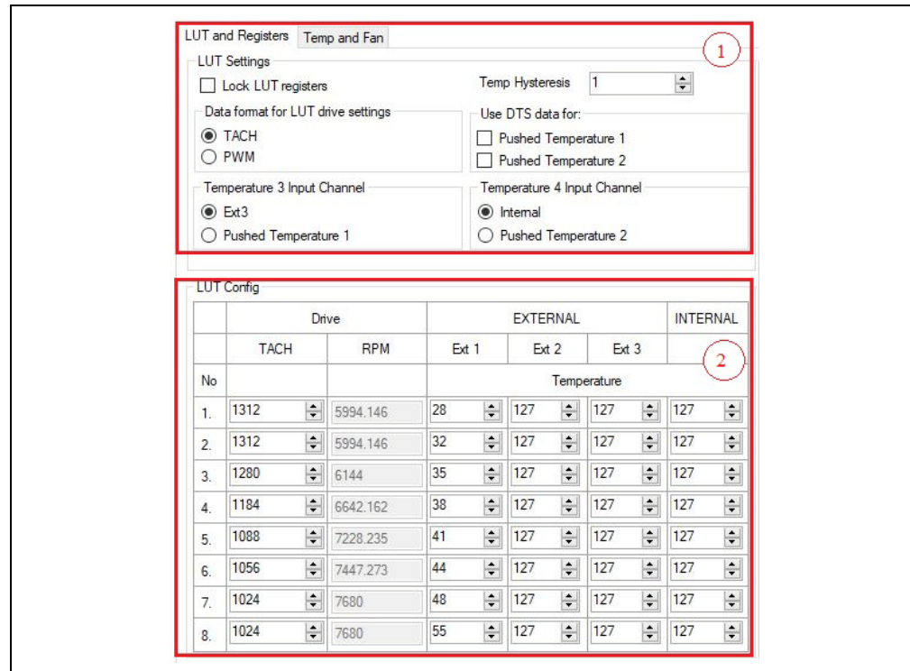
FIGURE 3-16: Look-up Table.
