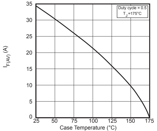
Figure 29. Maximum Average Forward Current vs. Case Temperature
