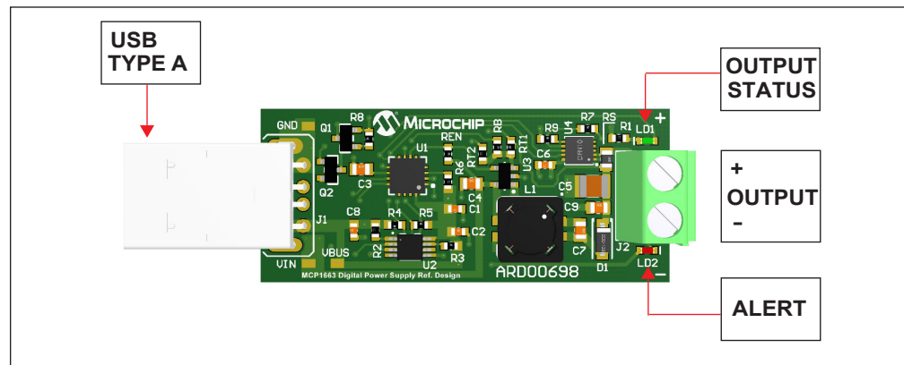
FIGURE 2-2: The MCP1663 USB Programmable Power Supply Overview.
