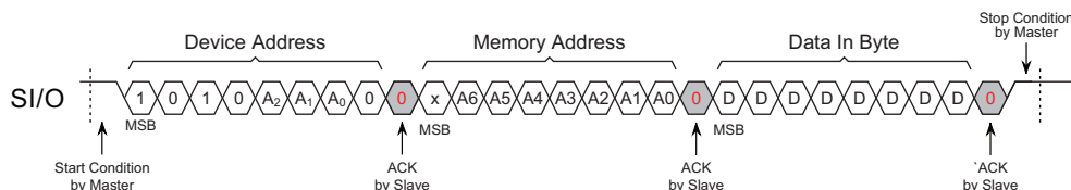
Figure 6-1. Byte Write
