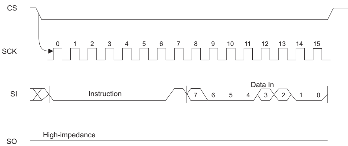
Figure 7-5. WRSR Timing
