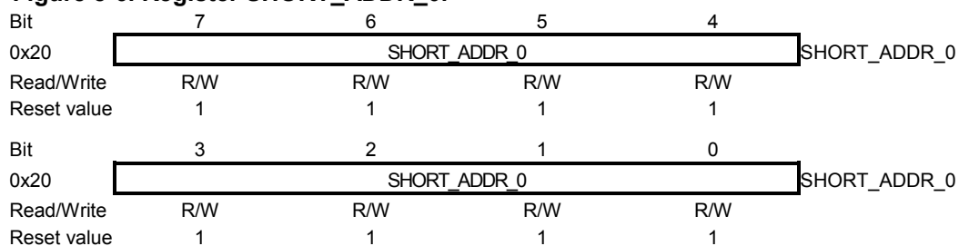
Figure 8-6. Register SHORT_ADDR_0.
