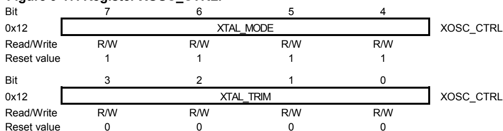
Figure 9-17. Register XOSC_CTRL.
