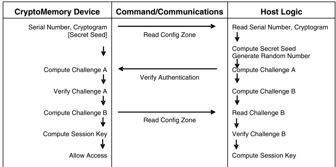
Figure 3. CryptoMemory Mutual Authentication
